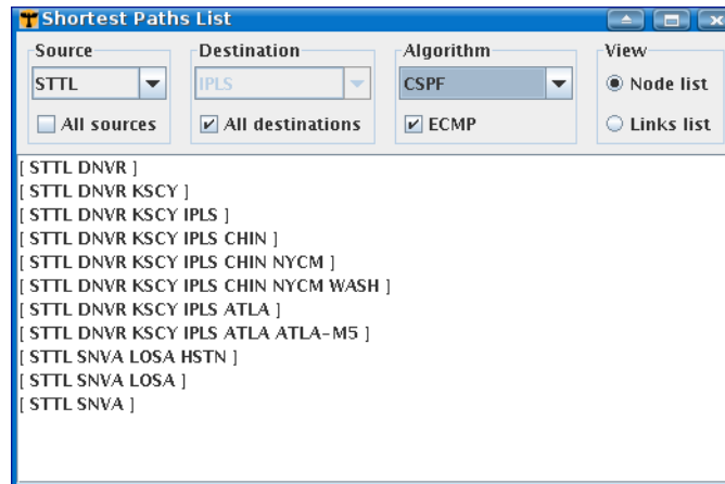
Figure 19: The list shortest paths dialog.
